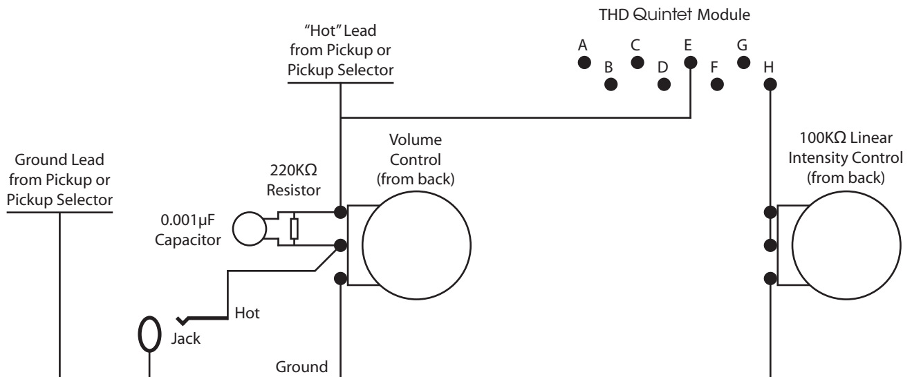
Typical installation using one setting as a replacement for regular tone control
