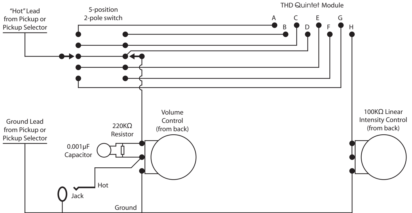
Typical installation using 5-position switch and intensity control
